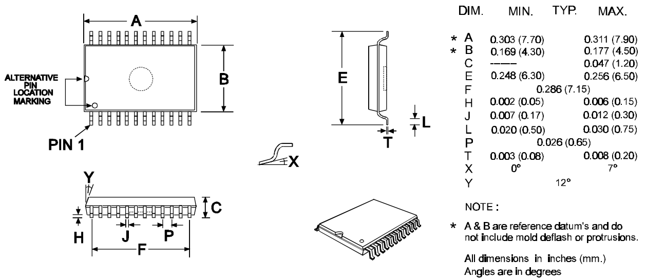
Figure 14b 24-pin TSSOP (E2) Mechanical Outline: Order as part no. CMX869E2
