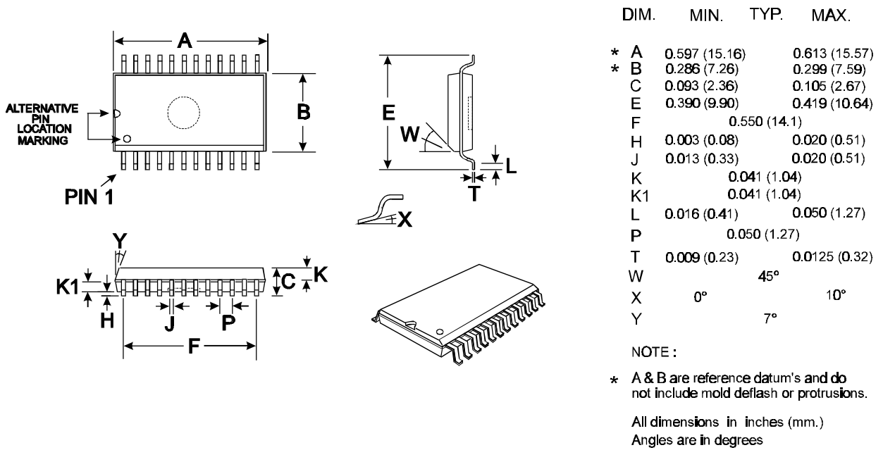
Figure 14a 24-pin SOIC (D2) Mechanical Outline: Order as part no. CMX869D2
