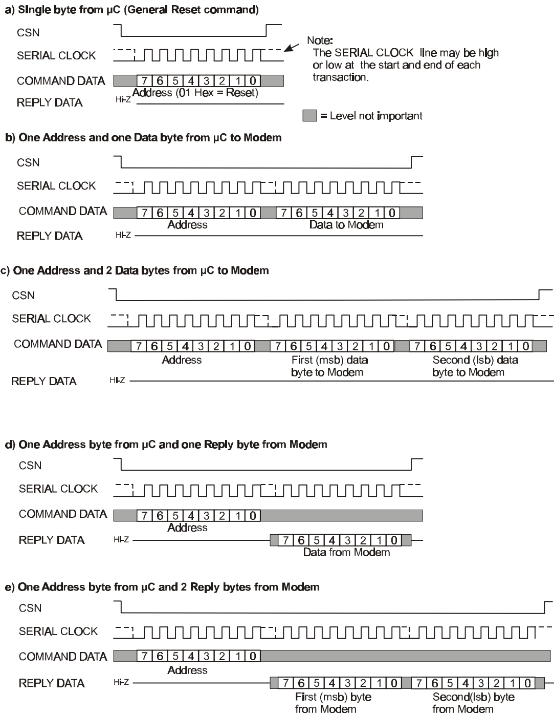
Figure 8 C-BUS Transactions
