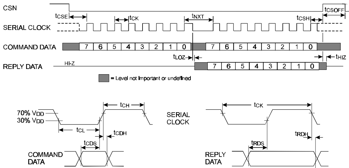
Figure 13 C-BUS Timing
