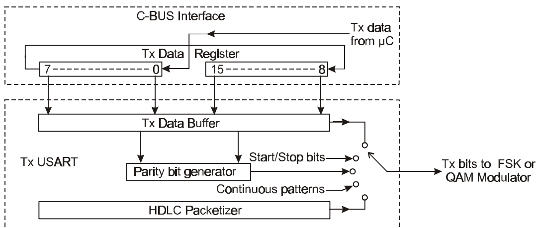
Figure 5a Tx USART (in 16 Bit Mode)
